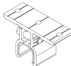
Klip-lok 700 clamp Material: Aluminum 6005 T5 Finish: Anodized
